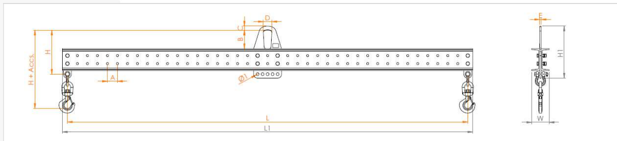
FIXED FRAME TYPE "A" WITH CENTERED LIFTING POINT
