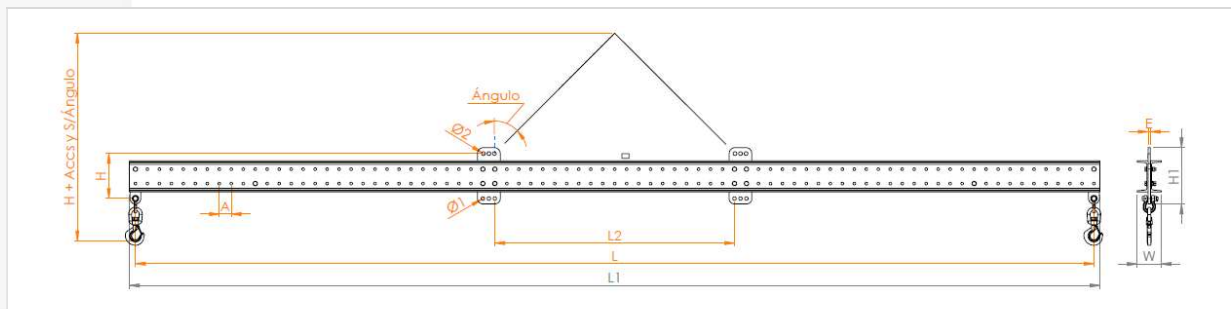
FIXED FRAME TYPE "B" WITH LIFTING POINTS FOR TWO-LEG SLINGS
